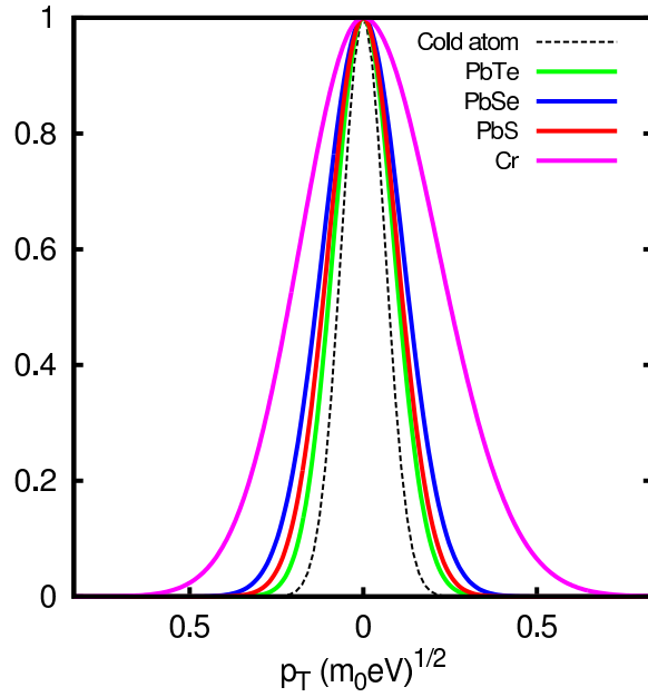
Figure 7.7: Comparison of transverse momentum distributions among the lead salt (111) faces, Cr(001) face and the cold atom source of Ref. [317].
